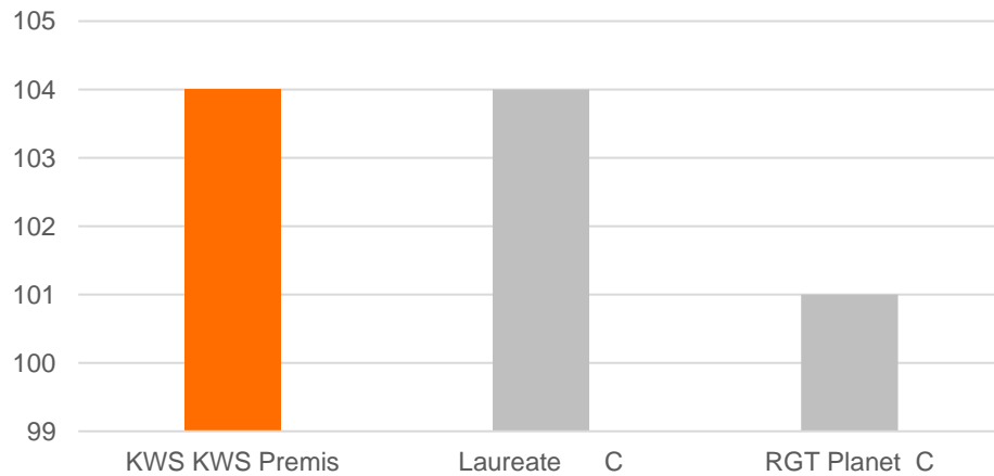
Sweden Yield relative (treated)
